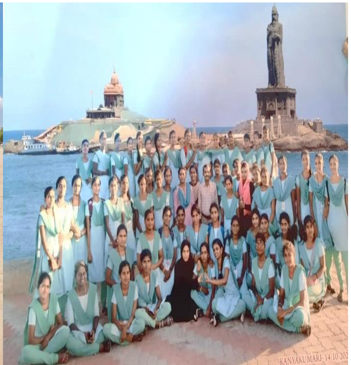
Beach Profile –Study of cross sectional trace of the beach perpendicular to the high tide shoreline which extends from the backshore cliff & Heavy Mineral Deposits along the sea shore at kanyakumari
